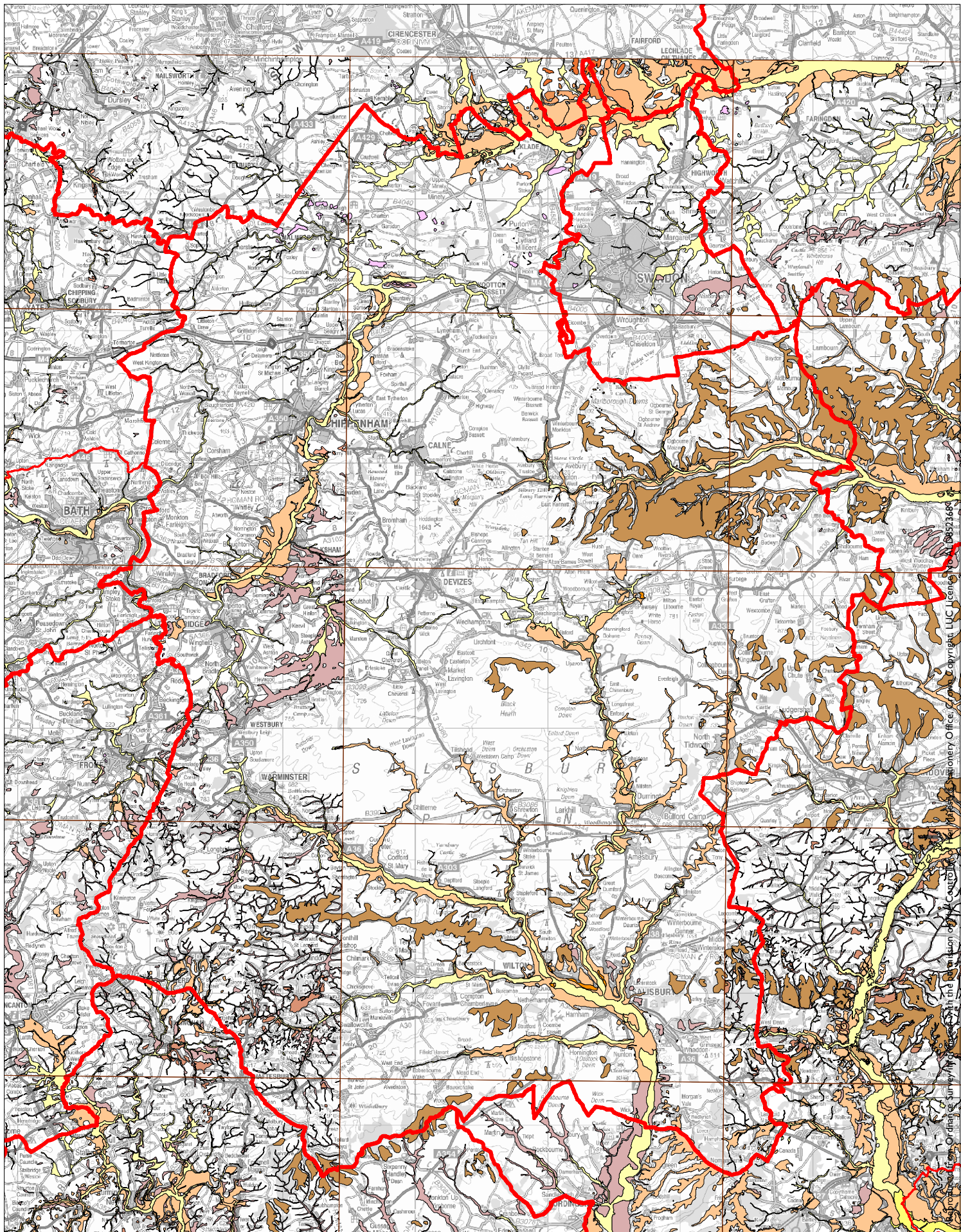
Figure 10: Drift Geology
